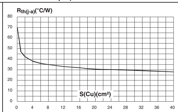
Figure 12. Thermal resistance junction to ambient versus copper surface under tab (Epoxy printed circuit board FR4, copper thickness: 35 µm)
